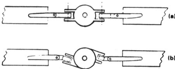
FIGURE 2-51. FLAPPING HINGES.
